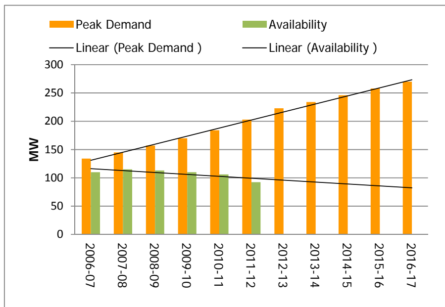
Figure 8: Demand & Availability of Power in Manipur
