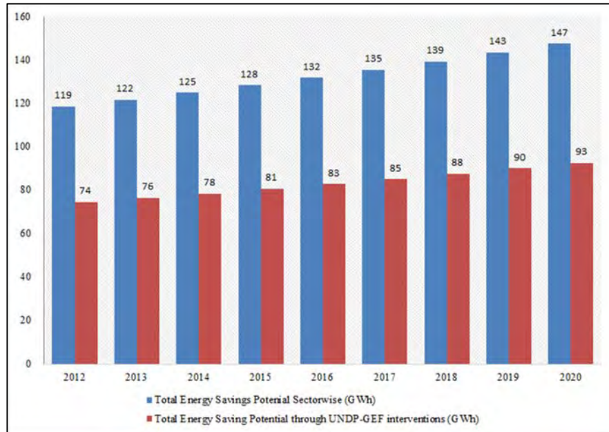
Figure 13: Energy Savings Projections- Manipur
