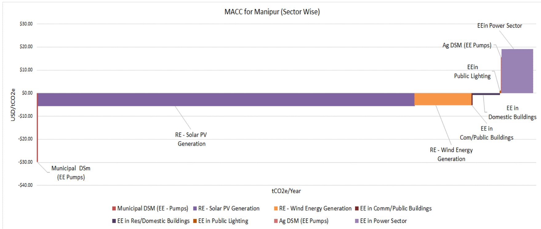
Figure 10: Sectoral MACC for State of Manipur
