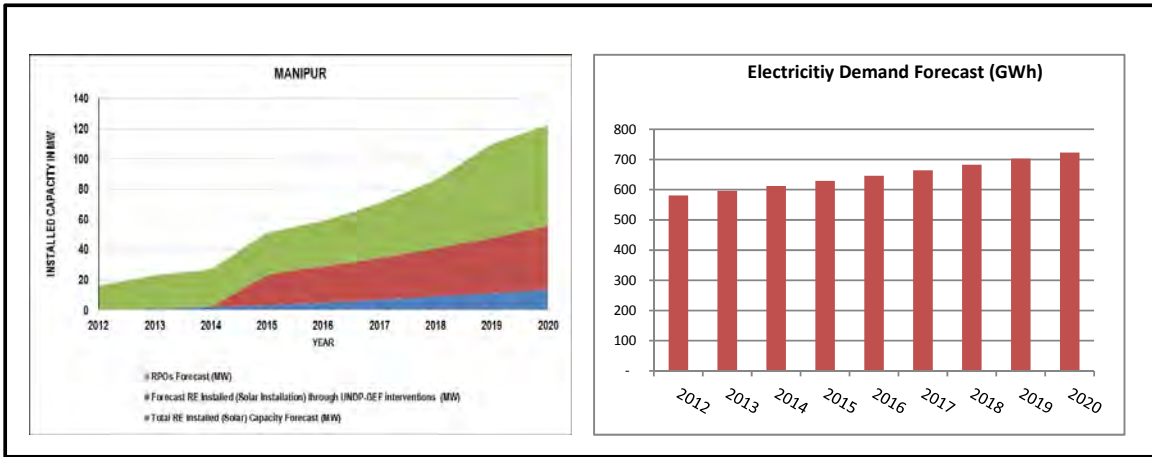
Figure 11: Manipur Renewable Energy's Scenarios
